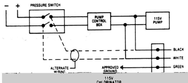
Figure 9 Wiring Diagram, 115 V Chlorinator, 115 V Well Pump
